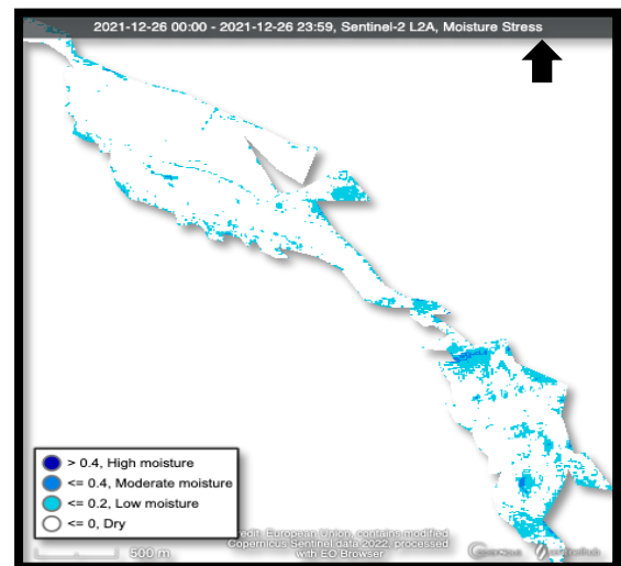
Figure 6 (ii): Moisture stress of Post (26 th December) Ain Marah wildfire (Copernicus 2022).
