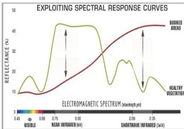
Figure 3. Comparison Of The Spectral Response Of Healthy Vegetation And Burned Areas (Keeley, 2009).
