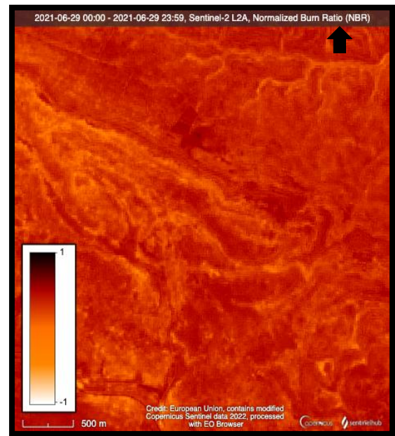
Figure 4. NBR of Pre (29th June) Ain Marah wildfire.
