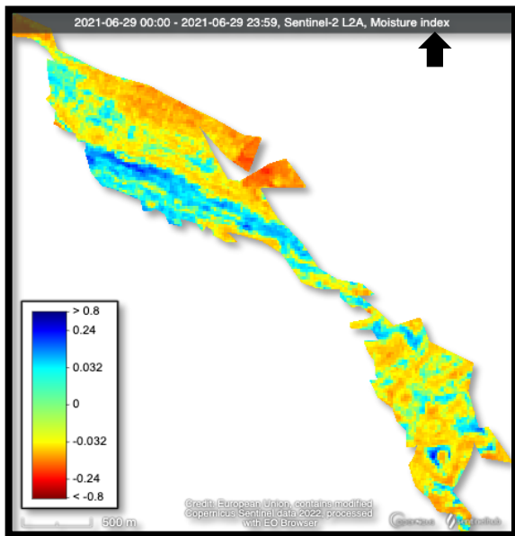
Figure 5 (i): NDMI of Pre (29th June) Ain Marah wildfire.
