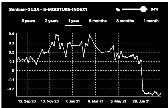
Chart 1: NDMI mean values variation from Aug 2020 to August 2021.
