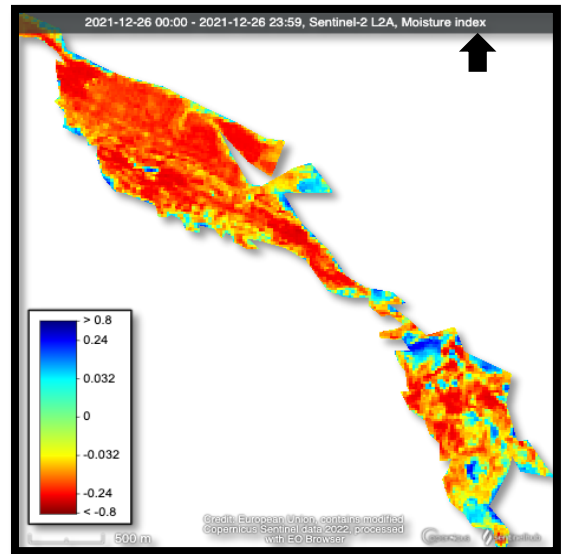
Figure 6 (i). NDMI of Post (26 th December) Ain Marah wildfire.
