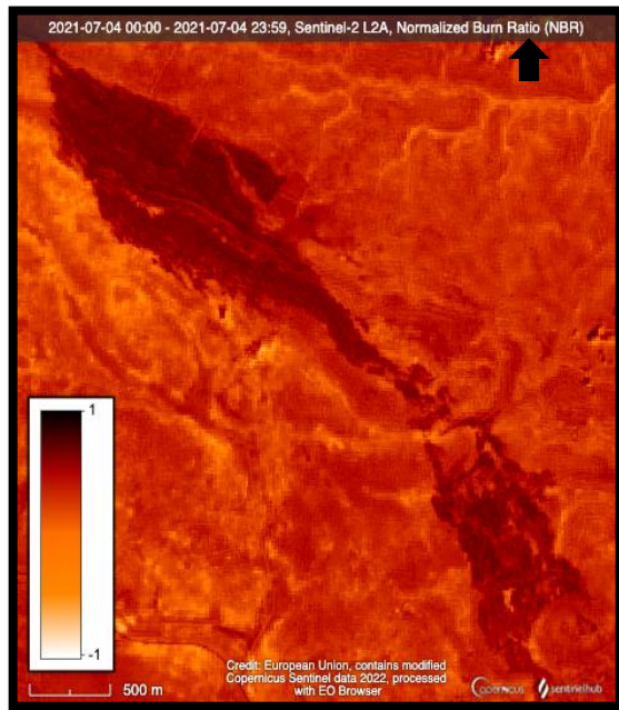
Figure 5. NBR of post Ain Marah wildfire (4 th July). [proceed by Copernicus 2021].
