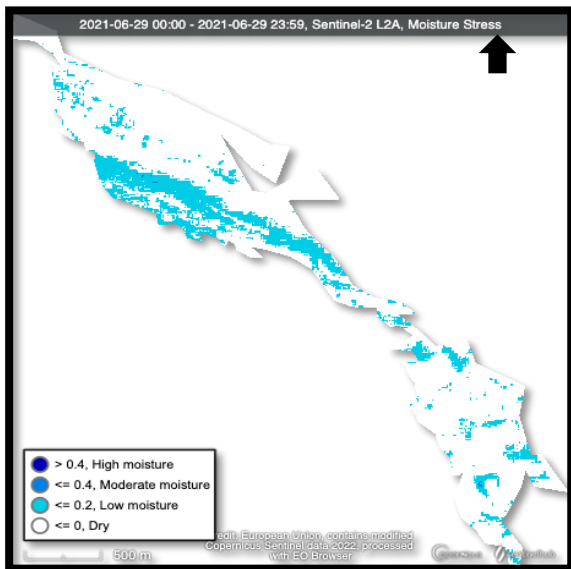
Figure 5 (ii): Moisture stress of Pre (29th June) Ain Marah wildfire [Copernicus 2022].
