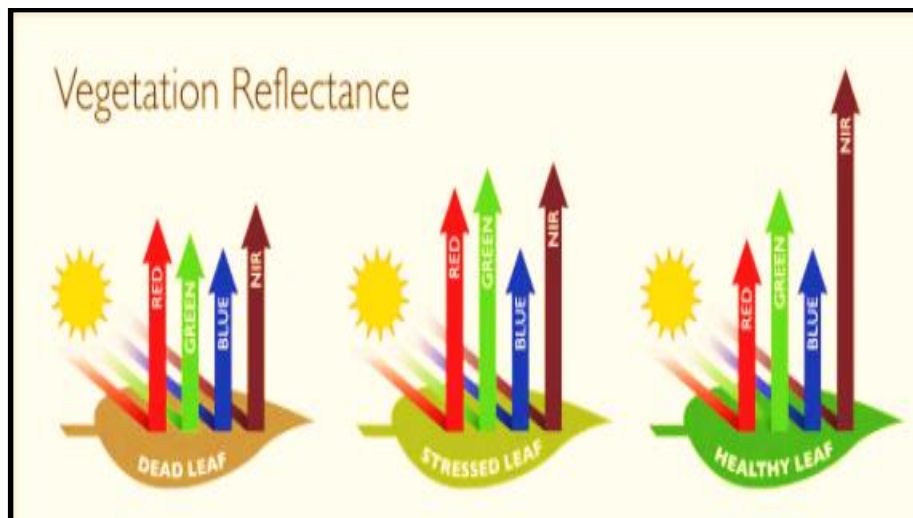
Figure 1: Vegetation indices with percentage of radiations emitted (Sara, 2018).
