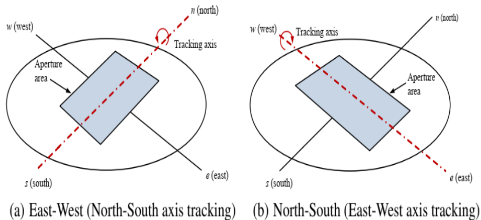
Figure 1: Tracking modes for PTC
