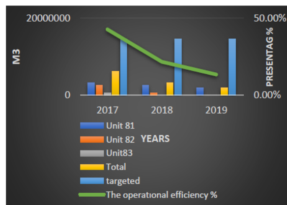
Figure 6. Diagram showing The Average quantities of desalinated water produced and the average operational efficiency % in Abu-Taraba Desalination Plant During the Period 2017-2019
